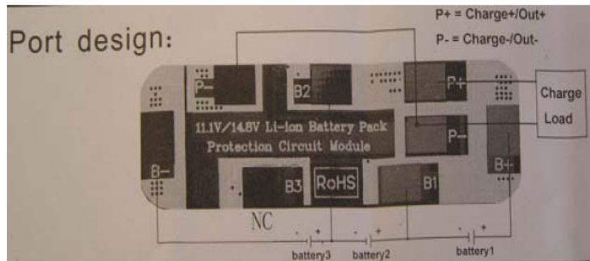
Picture 2: Port Design. (You need chose either two of P- point become the Charge-/out- terminal.)
